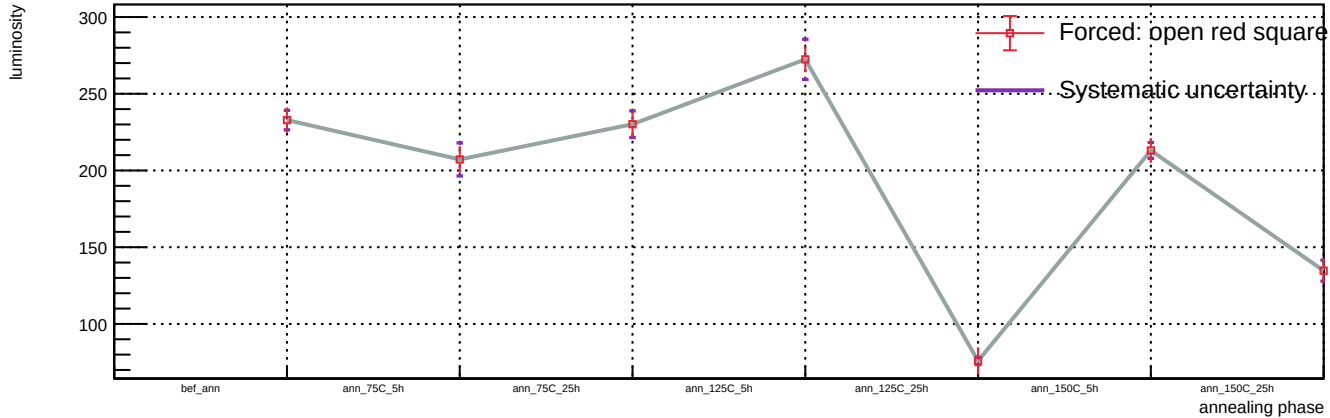
Sensor B1, v = 3 V, T = 23 °C - Spot 111: luminosity vs phase
