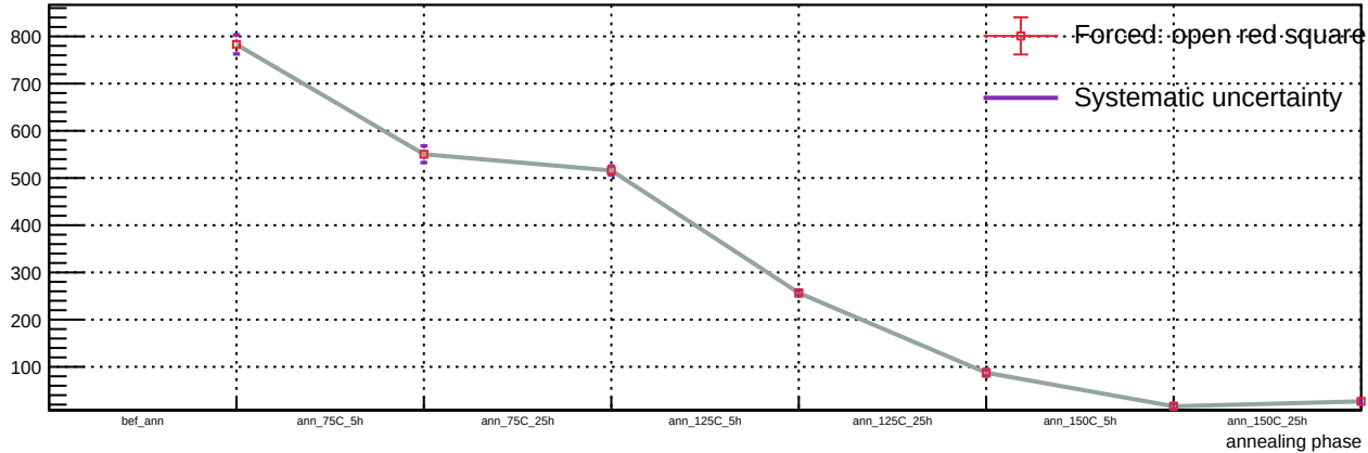
Sensor B1, v = 3 V, T = 23 °C - Spot 112: luminosity vs phase
