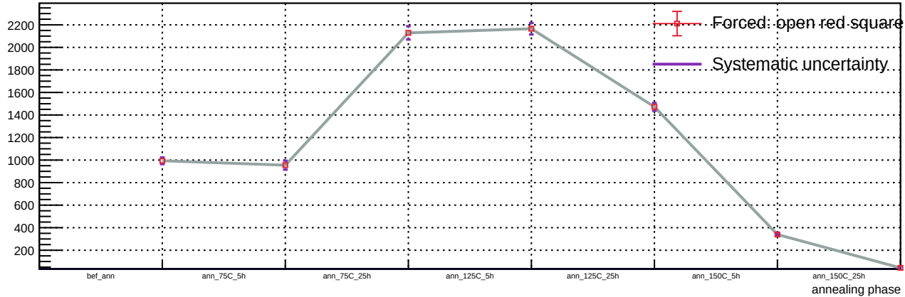
Sensor B1, v = 3 \text{ V} , T = 23 \text{ }^{\circ}\text{C} - Spot 114: luminosity vs phase
