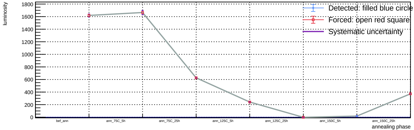
Sensor B1, v = 3 V, T = 23 °C - Spot 115: luminosity vs phase
