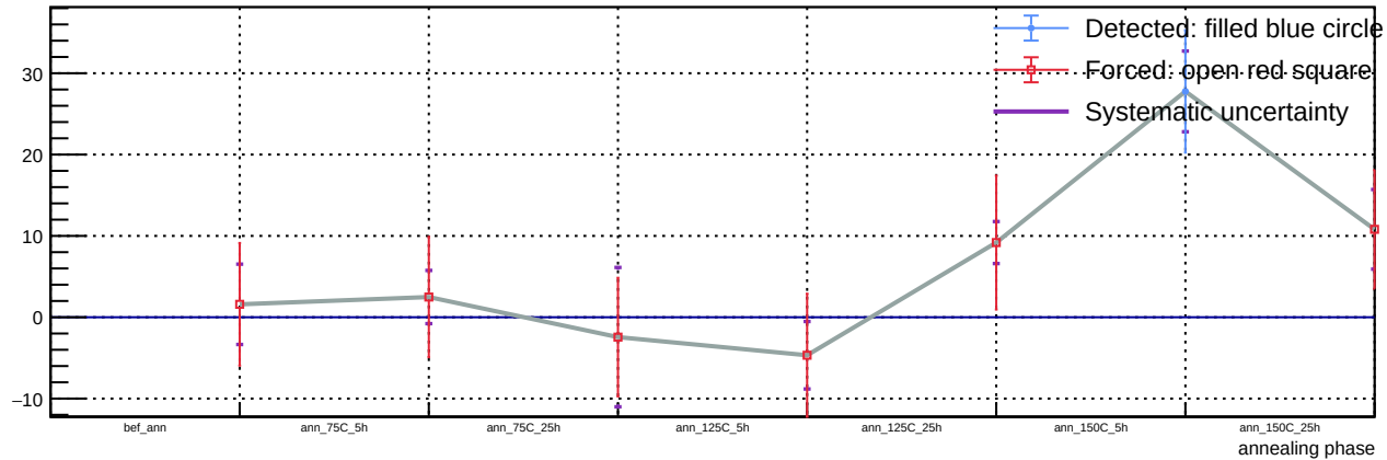
Sensor B1, v = 3 V, T = 23 °C - Spot 116: luminosity vs phase
