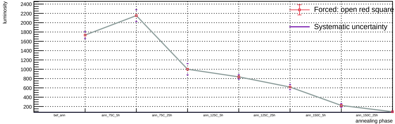
Sensor B1, v = 3 V, T = 23 °C - Spot 117: luminosity vs phase
