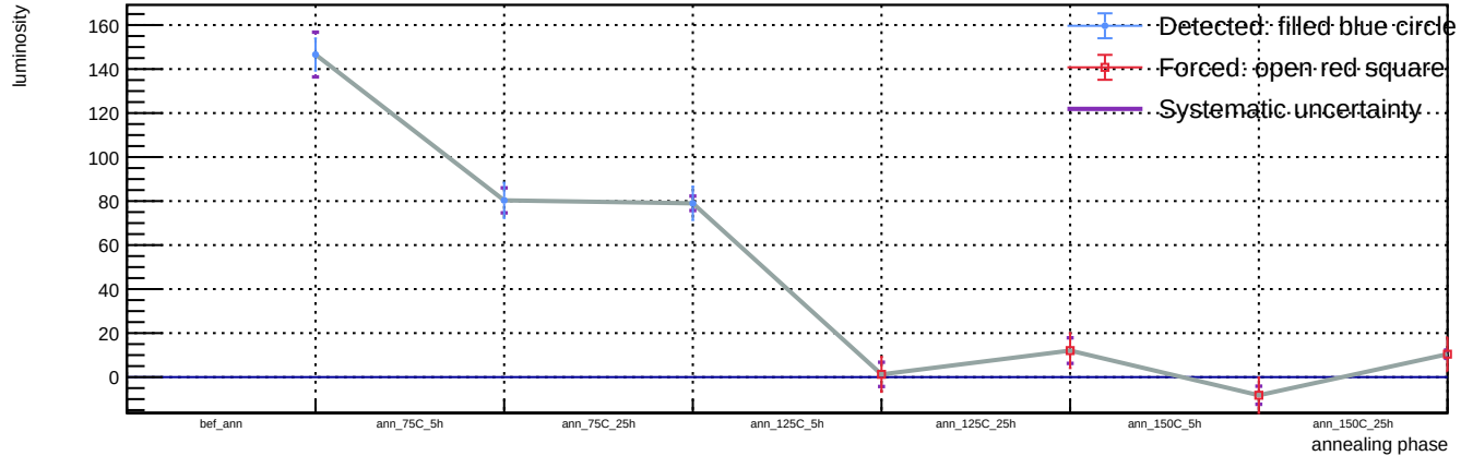
Sensor B1, v = 3 V, T = 23 °C - Spot 13: luminosity vs phase
