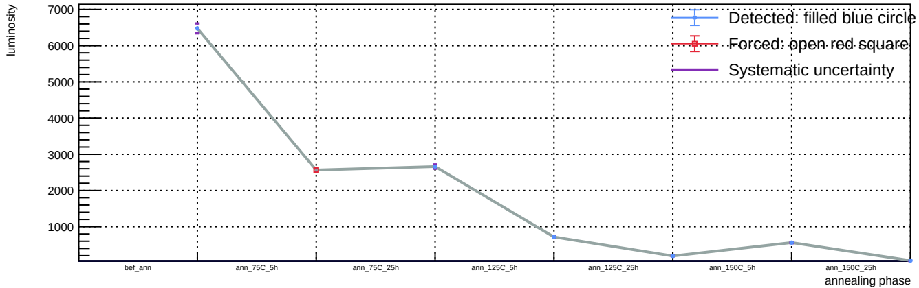
Sensor B1, v = 3 \text{ V} , T = 23 \text{ }^{\circ}\text{C} - Spot 14: luminosity vs phase
