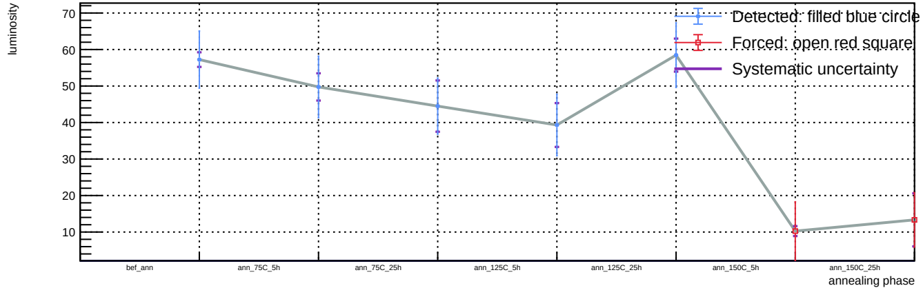
Sensor B1, v = 3 V, T = 23 °C - Spot 15: luminosity vs phase
