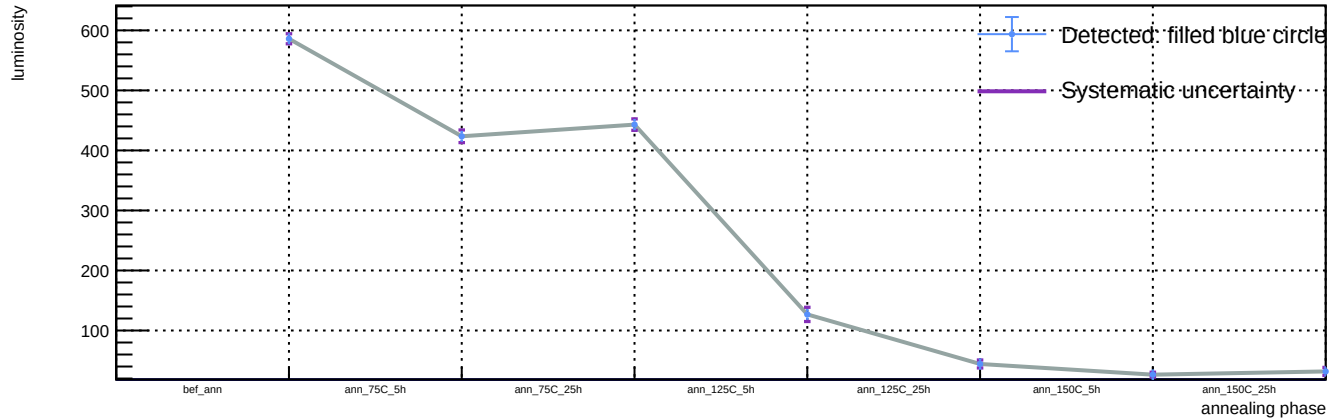
Sensor B1, v = 3 V, T = 23 °C - Spot 18: luminosity vs phase
