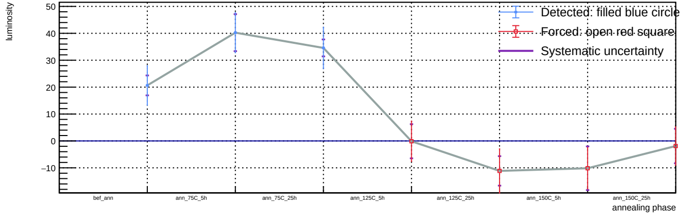
Sensor B1, v = 3 \text{ V} , T = 23 \text{ }^{\circ}\text{C} - Spot 19: luminosity vs phase
