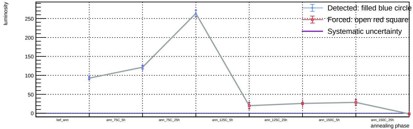
Sensor B1, v = 3 V, T = 23 °C - Spot 2: luminosity vs phase
