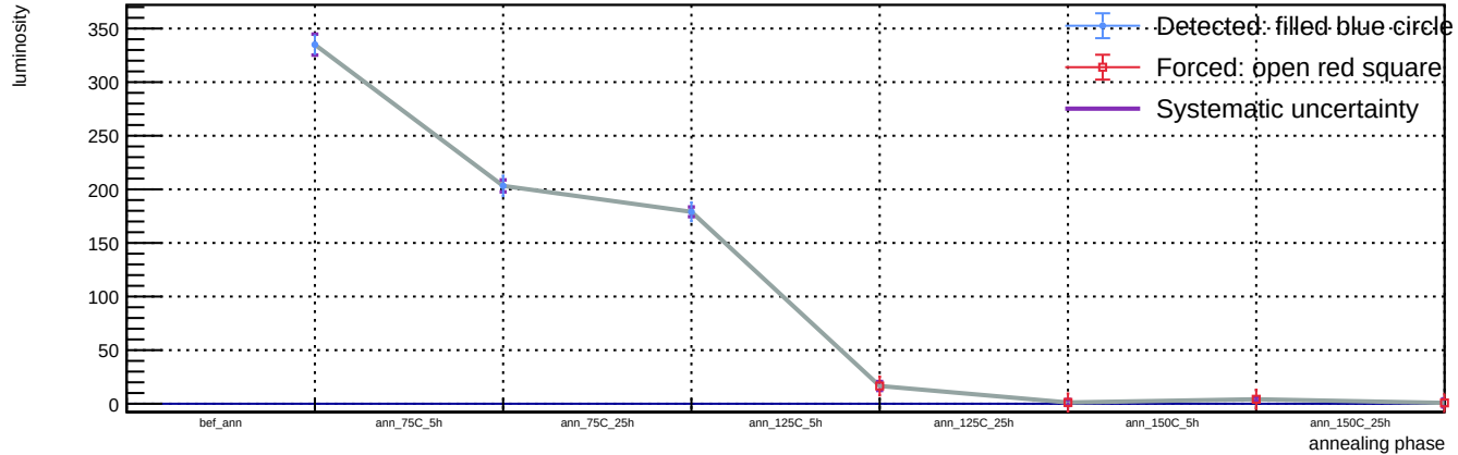
Sensor B1, v = 3 V, T = 23 °C - Spot 20: luminosity vs phase
