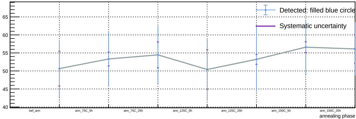
Sensor B1, v = 3 V, T = 23 °C - Spot 21: luminosity vs phase
