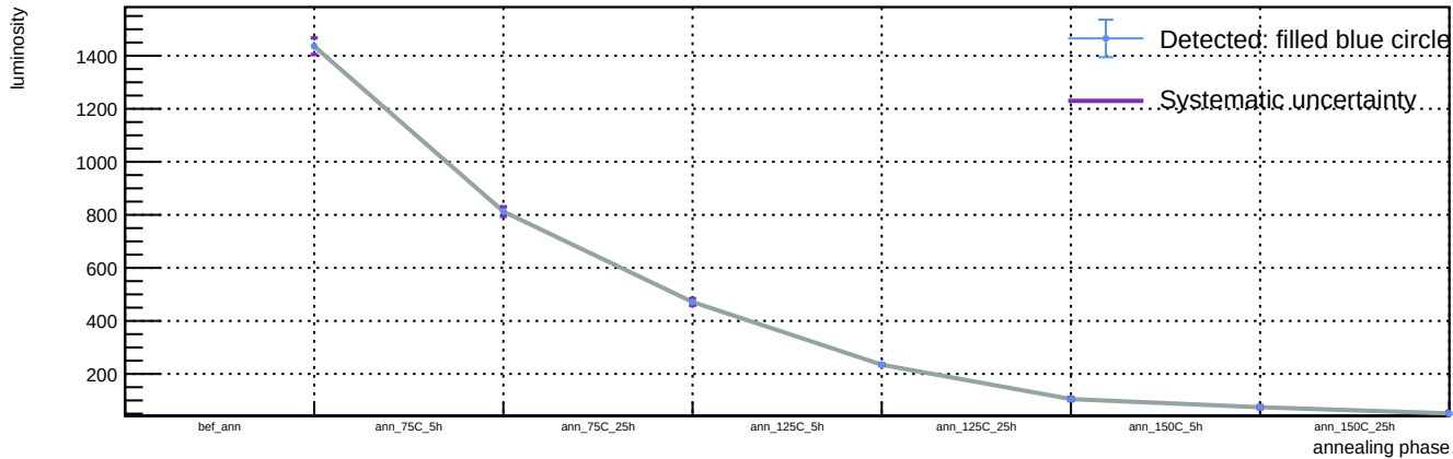
Sensor B1, v = 3 V, T = 23 °C - Spot 23: luminosity vs phase
