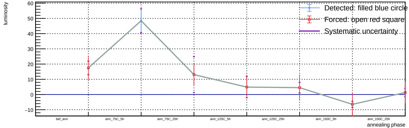
Sensor B1, v = 3 V, T = 23 °C - Spot 24: luminosity vs phase
