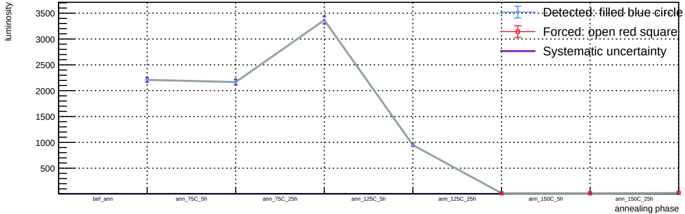
Sensor B1, v = 3 \text{ V} , T = 23 \text{ }^{\circ}\text{C} - Spot 25: luminosity vs phase
