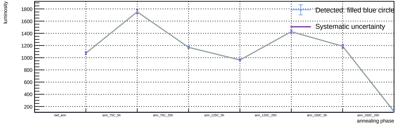
Sensor B1, v = 3 V, T = 23 °C - Spot 26: luminosity vs phase
