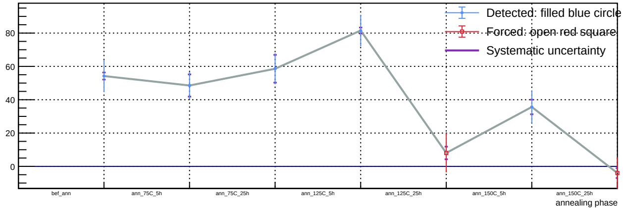
Sensor B1, v = 3 V, T = 23 °C - Spot 27: luminosity vs phase
