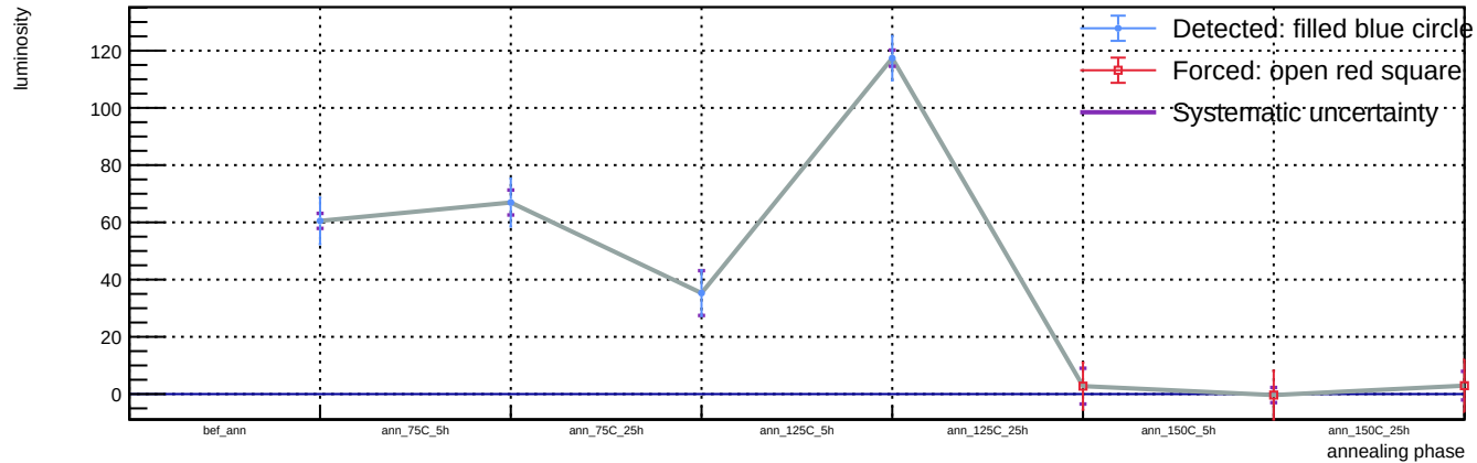
Sensor B1, v = 3 V, T = 23 °C - Spot 28: luminosity vs phase
