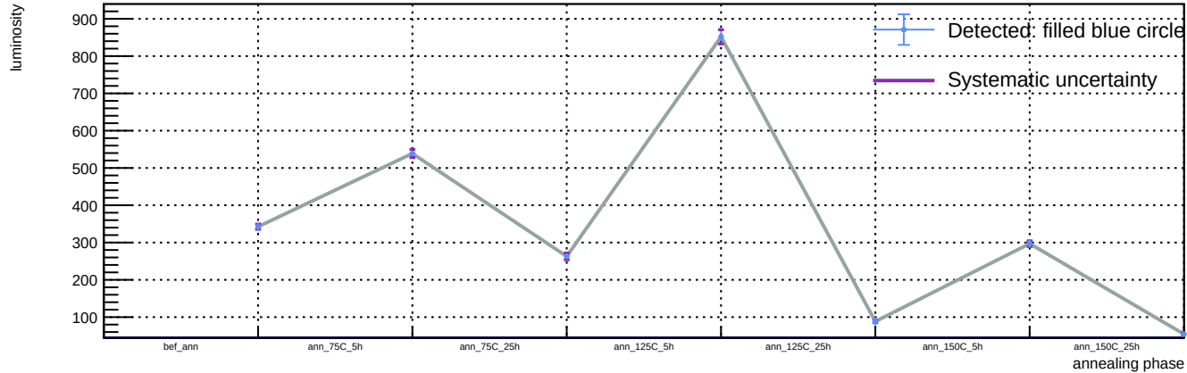
Sensor B1, v = 3 V, T = 23 °C - Spot 29: luminosity vs phase
