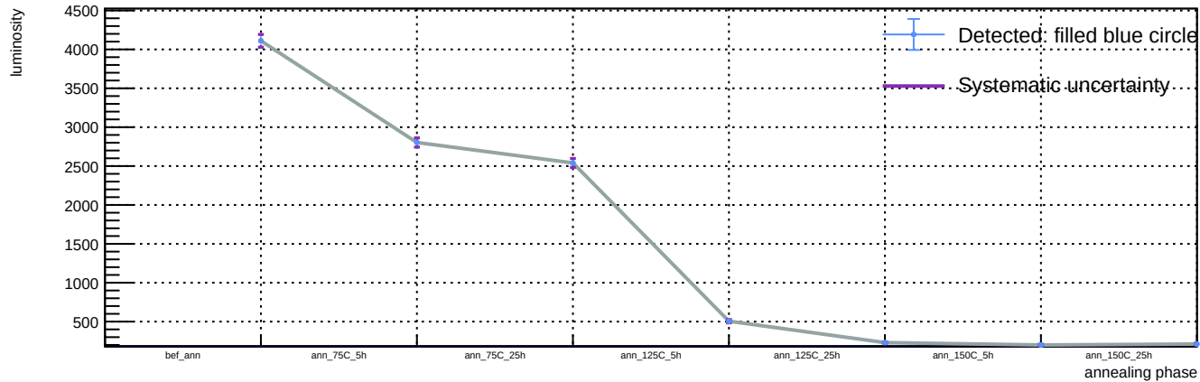
Sensor B1, v = 3 \text{ V} , T = 23 \text{ }^{\circ}\text{C} - Spot 30: luminosity vs phase
