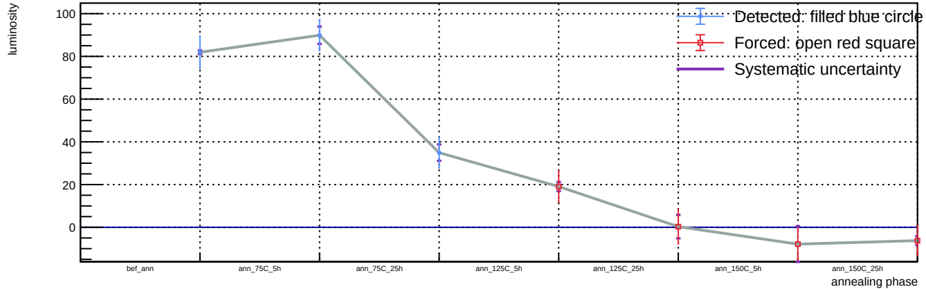
Sensor B1, v = 3 V, T = 23 °C - Spot 32: luminosity vs phase
