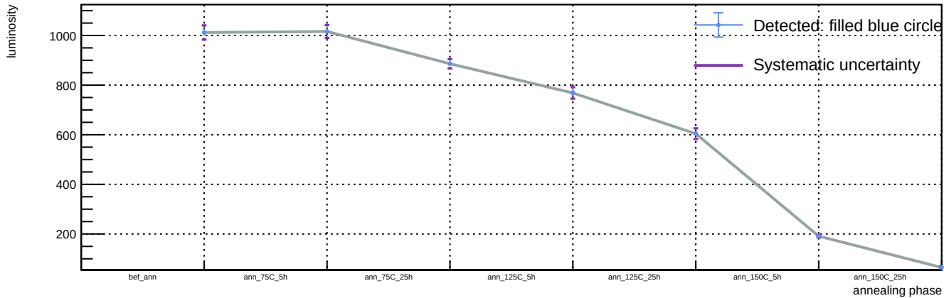
Sensor B1, v = 3 V, T = 23 °C - Spot 34: luminosity vs phase
