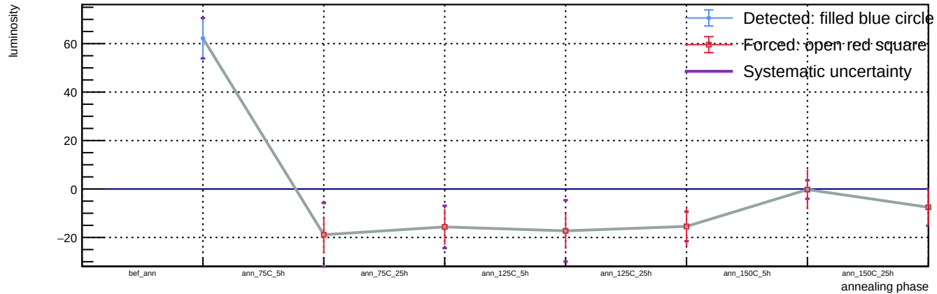
Sensor B1, v = 3 V, T = 23 °C - Spot 35: luminosity vs phase
