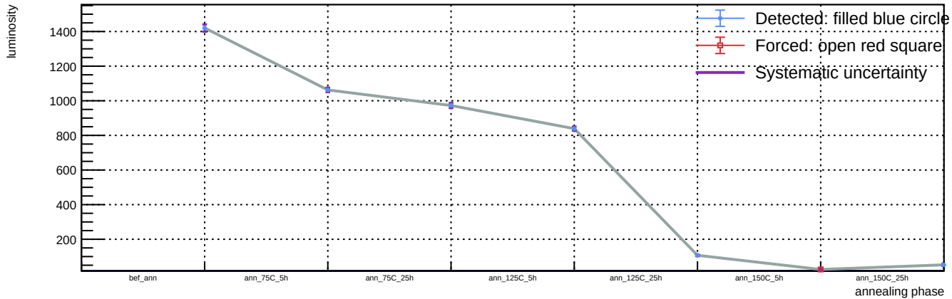
Sensor B1, v = 3 V, T = 23 °C - Spot 36: luminosity vs phase
