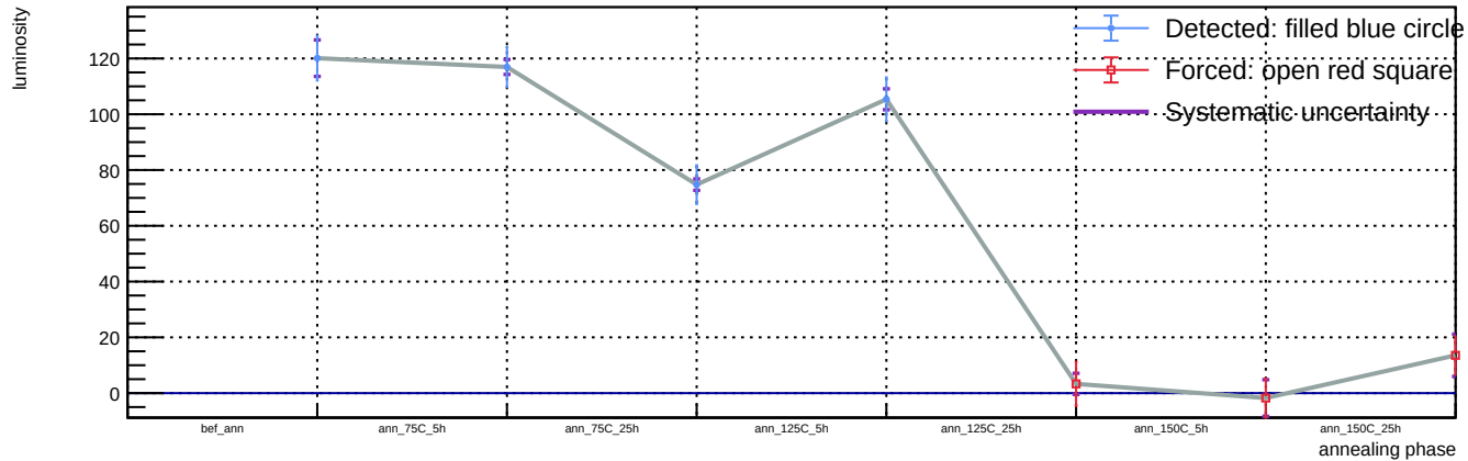
Sensor B1, v = 3 V, T = 23 °C - Spot 38: luminosity vs phase
