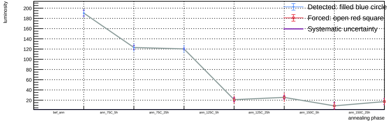
Sensor B1, v = 3 V, T = 23 °C - Spot 39: luminosity vs phase
