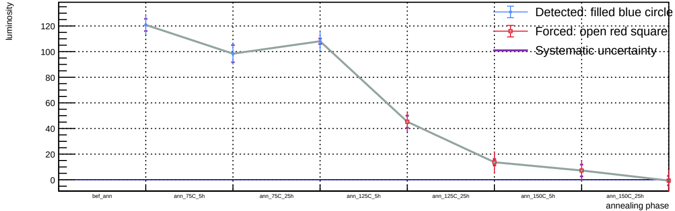
Sensor B1, v = 3 V, T = 23 °C - Spot 4: luminosity vs phase
