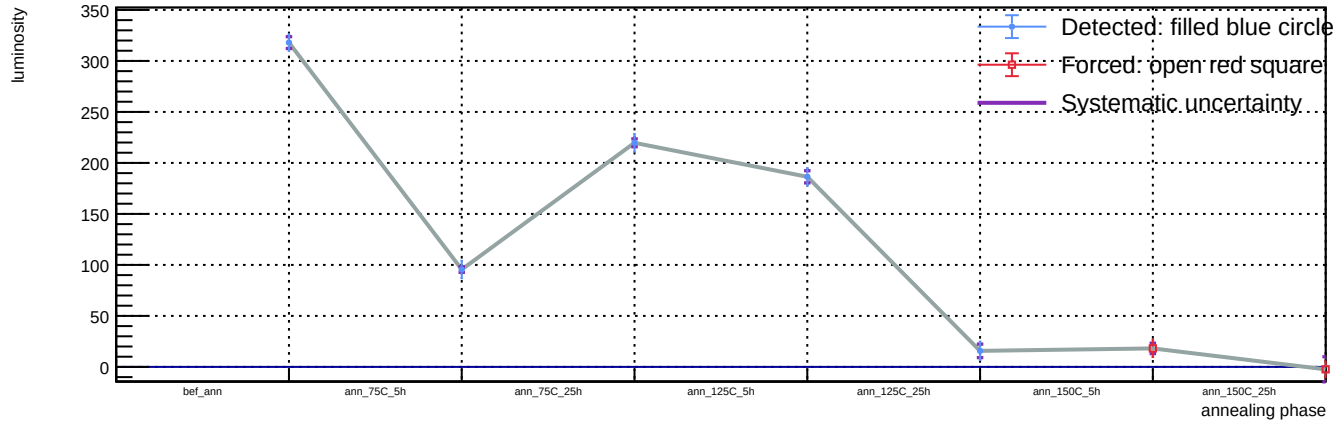
Sensor B1, v = 3 V, T = 23 °C - Spot 40: luminosity vs phase
