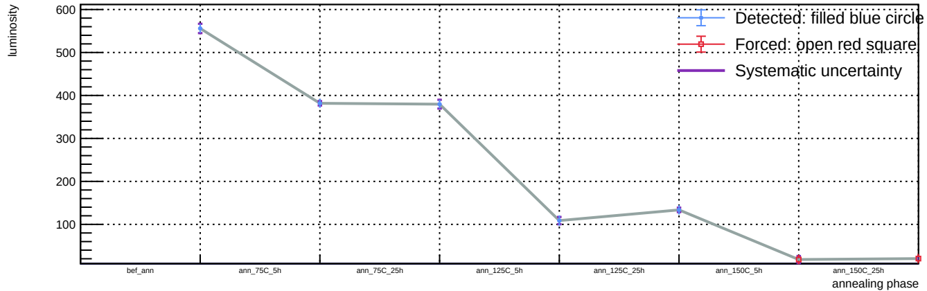
Sensor B1, v = 3 V, T = 23 °C - Spot 42: luminosity vs phase
