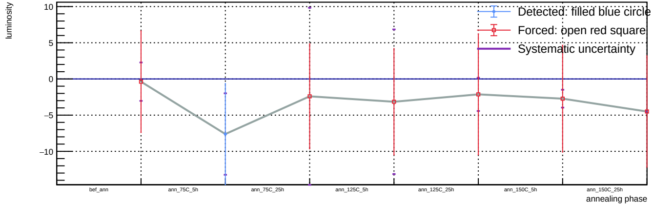
Sensor B1, v = 3 V, T = 23 °C - Spot 43: luminosity vs phase
