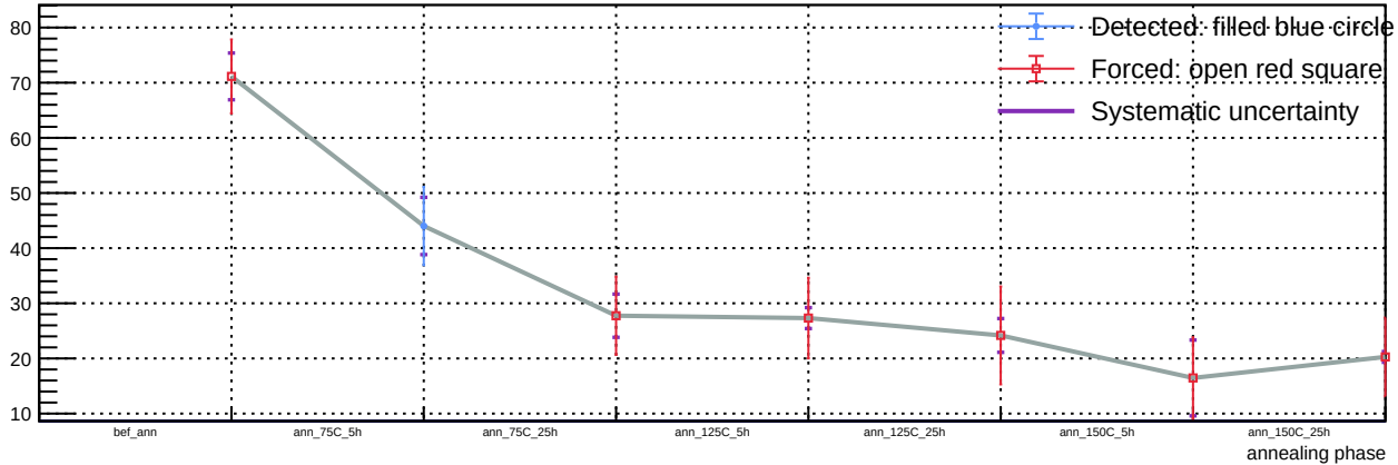
Sensor B1, v = 3\text{ V} , T = 23\text{ }^{\circ}\text{C} - Spot 44: luminosity vs phase
