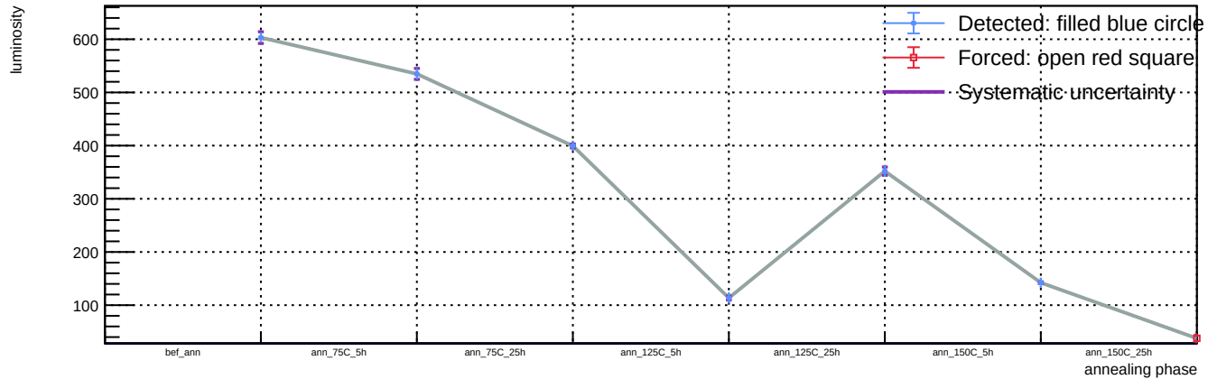
Sensor B1, v = 3 V, T = 23 °C - Spot 45: luminosity vs phase
