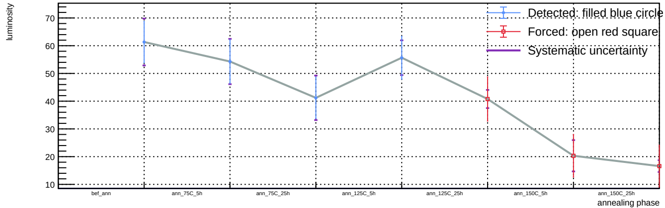
Sensor B1, v = 3 V, T = 23 °C - Spot 46: luminosity vs phase
