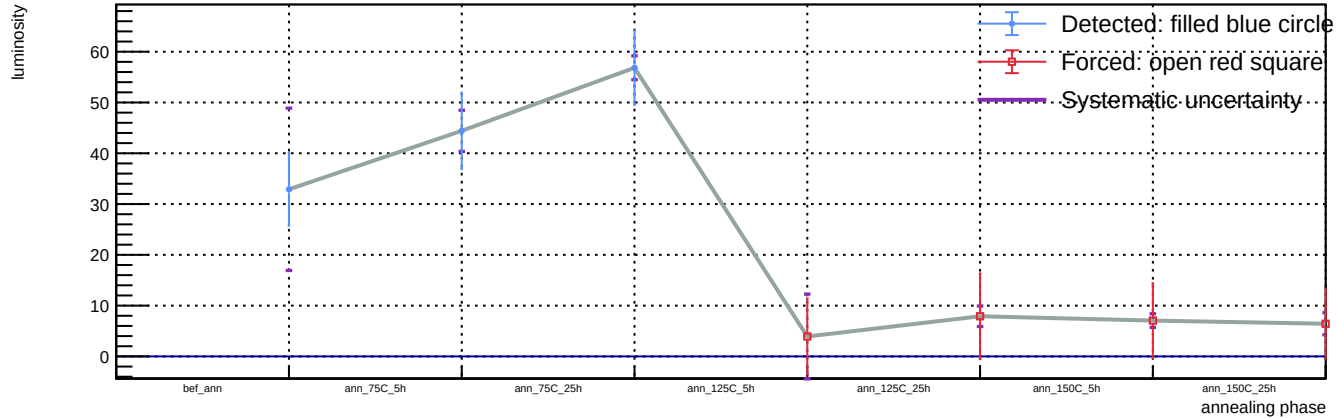
Sensor B1, v = 3 V, T = 23 °C - Spot 47: luminosity vs phase
