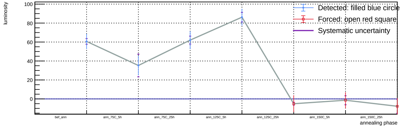
Sensor B1, v = 3 V, T = 23 °C - Spot 48: luminosity vs phase
