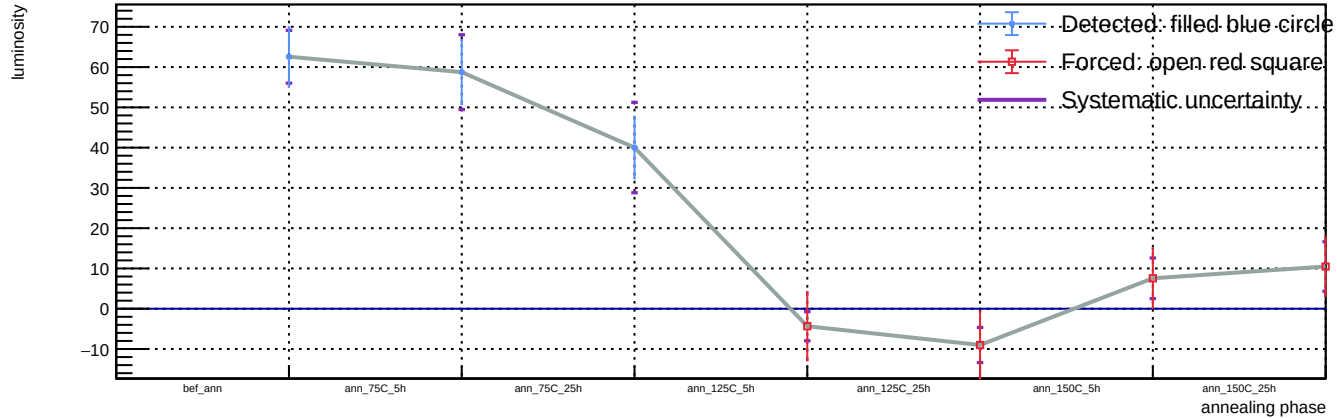
Sensor B1, v = 3 \text{ V} , T = 23 \text{ }^{\circ}\text{C} - Spot 49: luminosity vs phase
