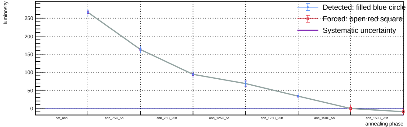
Sensor B1, v = 3 V, T = 23 °C - Spot 5: luminosity vs phase
