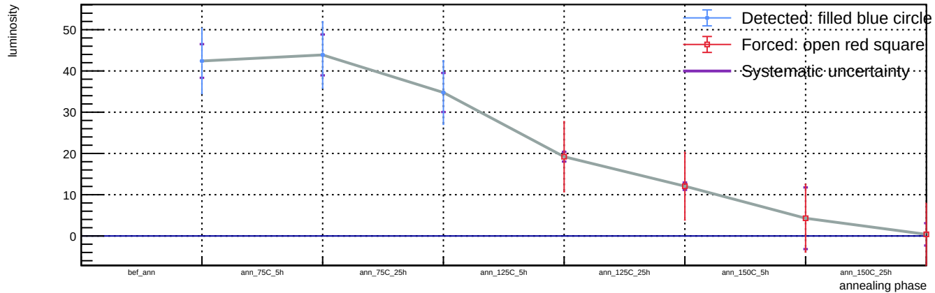
Sensor B1, v = 3 V, T = 23 °C - Spot 50: luminosity vs phase
