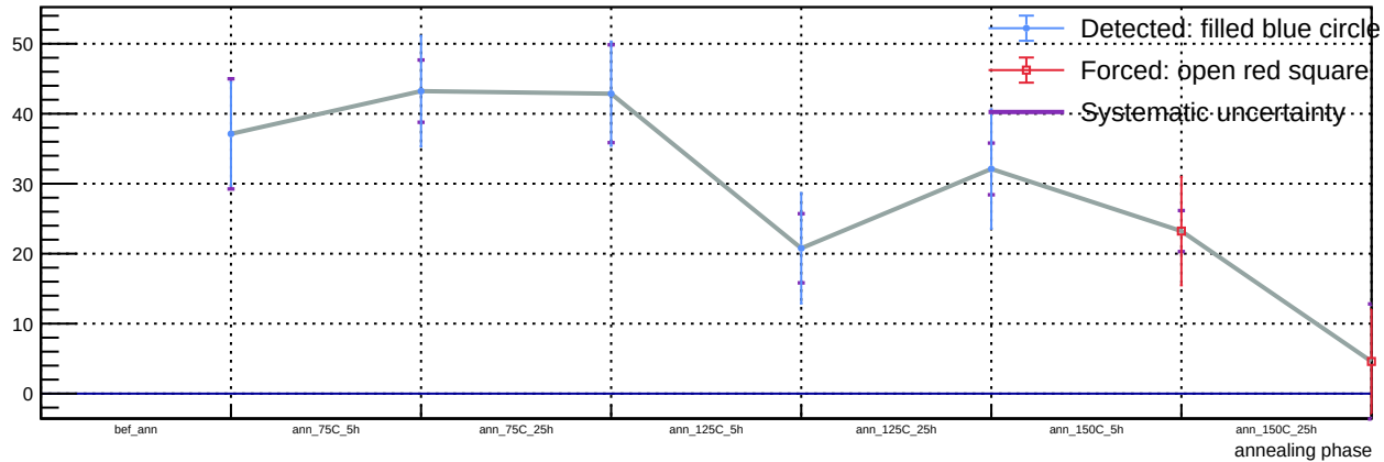
Sensor B1, v = 3 \text{ V} , T = 23 \text{ }^{\circ}\text{C} - Spot 51: luminosity vs phase
