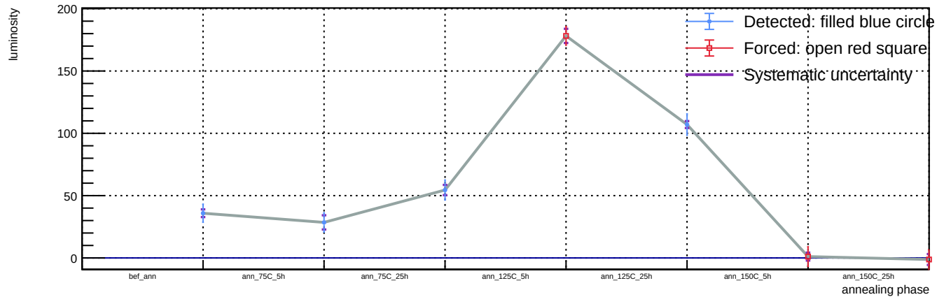
Sensor B1, v = 3 V, T = 23 °C - Spot 52: luminosity vs phase
