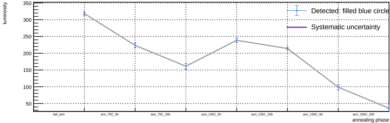
Sensor B1, v = 3 V, T = 23 °C - Spot 53: luminosity vs phase
