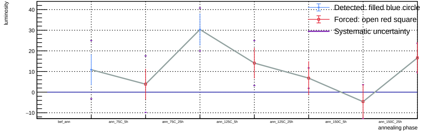
Sensor B1, v = 3 V, T = 23 °C - Spot 54: luminosity vs phase
