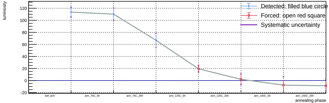
Sensor B1, v = 3 V, T = 23 °C - Spot 55: luminosity vs phase
