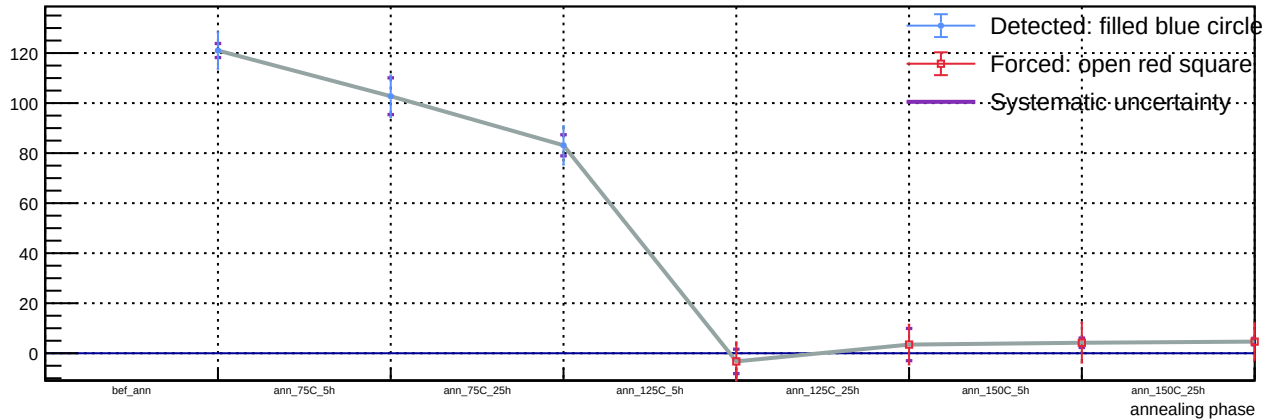
Sensor B1, v = 3 V, T = 23 °C - Spot 56: luminosity vs phase
