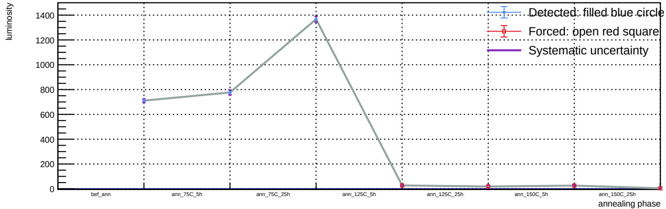
Sensor B1, v = 3 V, T = 23 °C - Spot 59: luminosity vs phase
