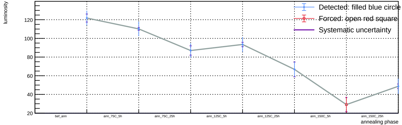
Sensor B1, v = 3 V, T = 23 °C - Spot 6: luminosity vs phase
