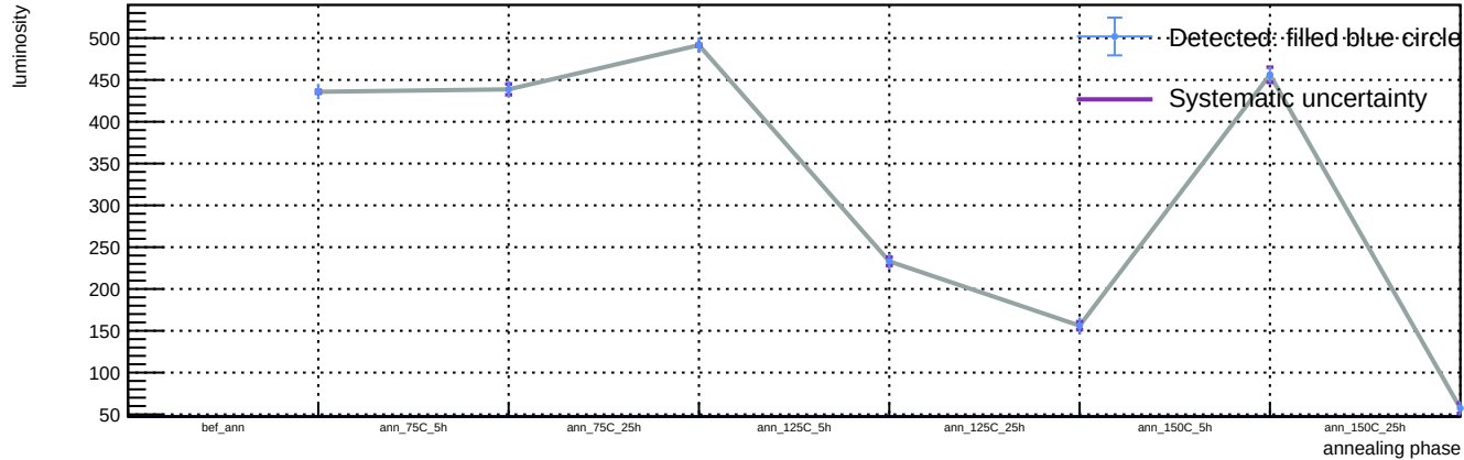
Sensor B1, v = 3 \text{ V} , T = 23 \text{ }^{\circ}\text{C} - Spot 60: luminosity vs phase
