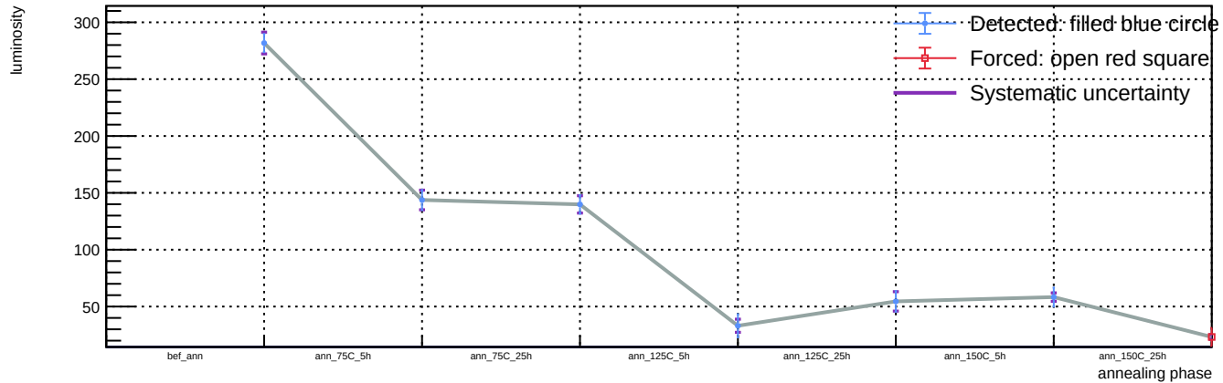
Sensor B1, v = 3\text{ V} , T = 23\text{ }^{\circ}\text{C} - Spot 61: luminosity vs phase
